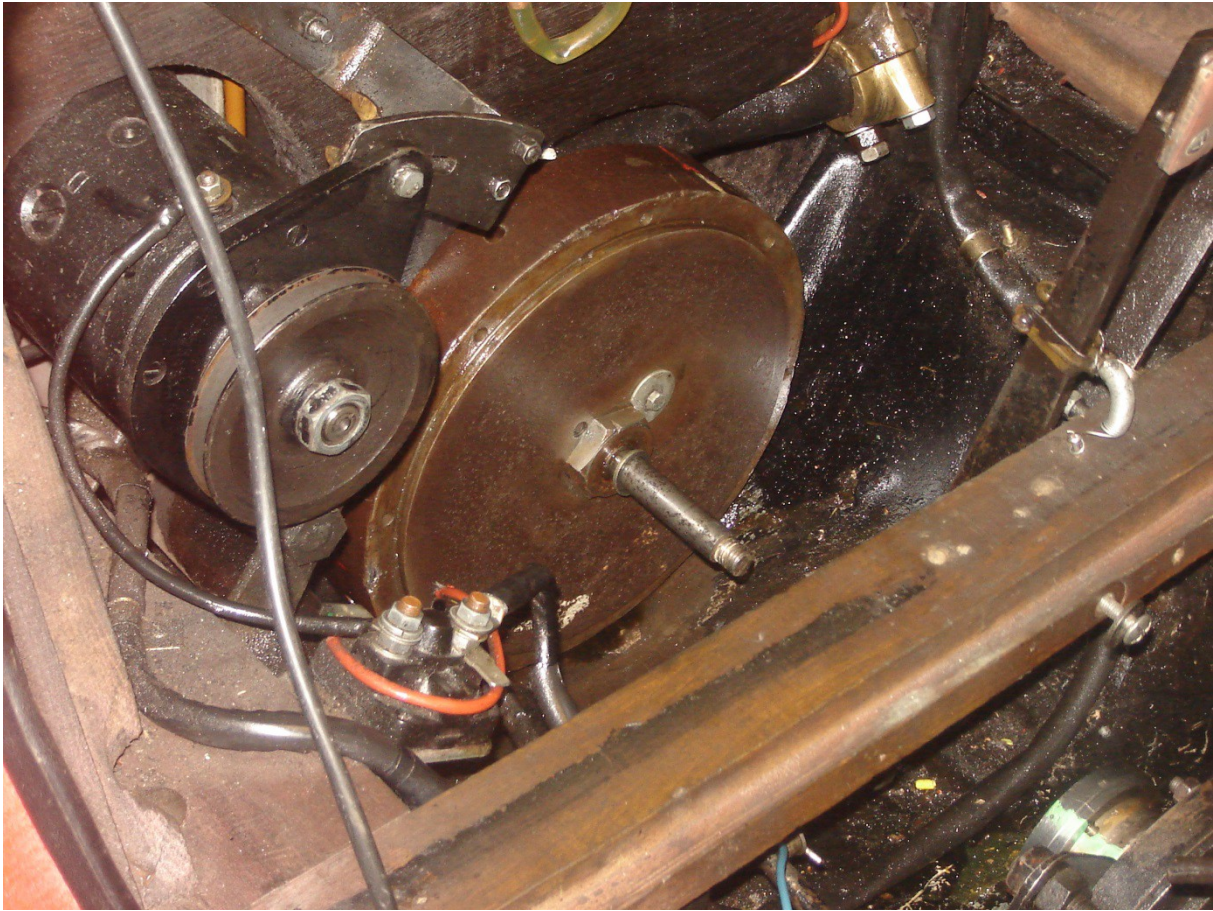
Peugeot bebe 1913 clutch flywheel
